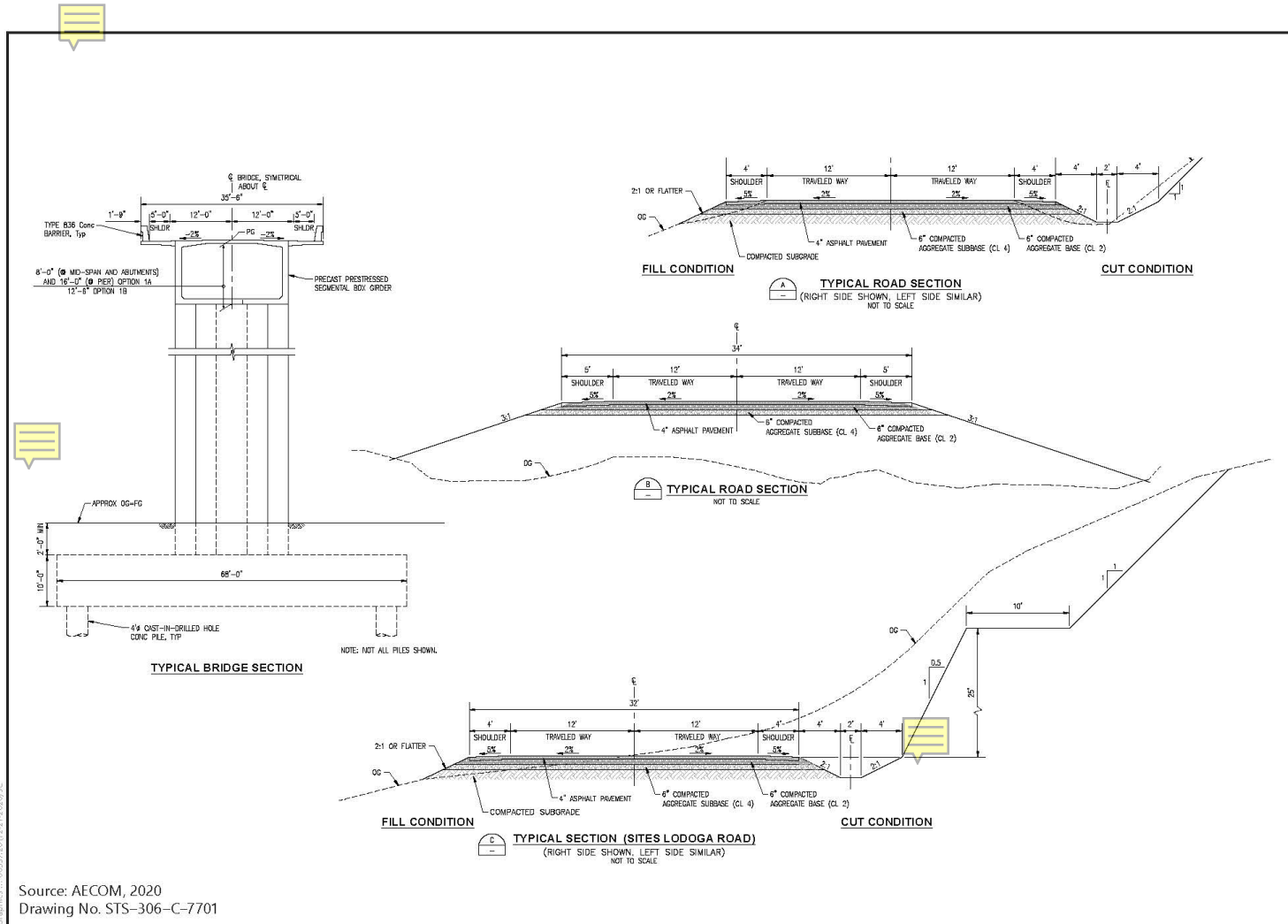
Figure 2-40. Sites Lodoga Road Realignment and Bridge
