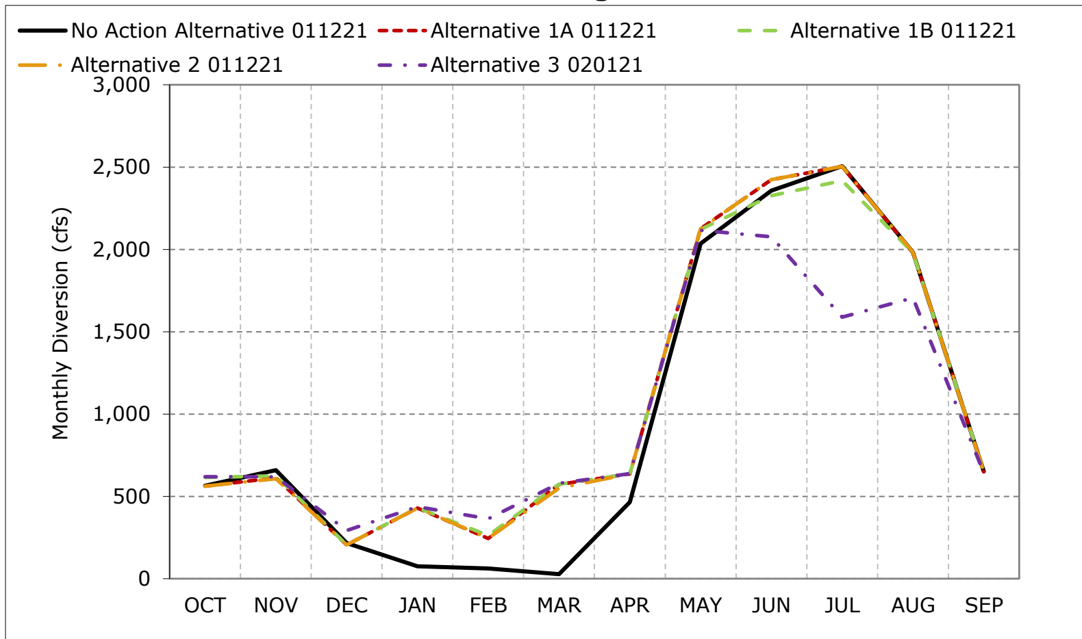
Figure 5C-4-3. Hamilton City Diversion - Glenn Colusa Canal, Above Normal Year Average Diversion
