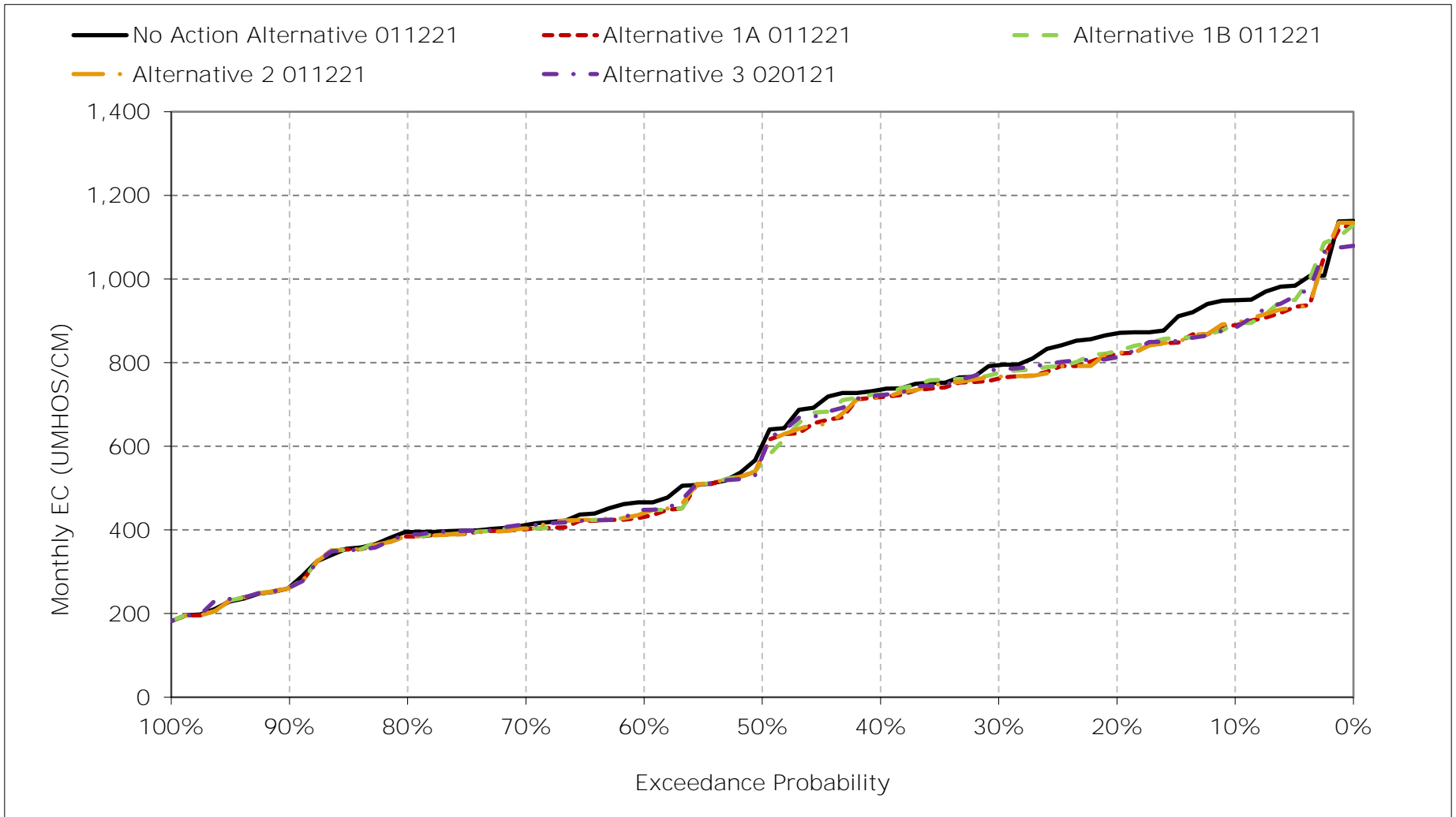
Figure 6B1-13-17. San Joaquin River at San Andreas Salinity, November EC
