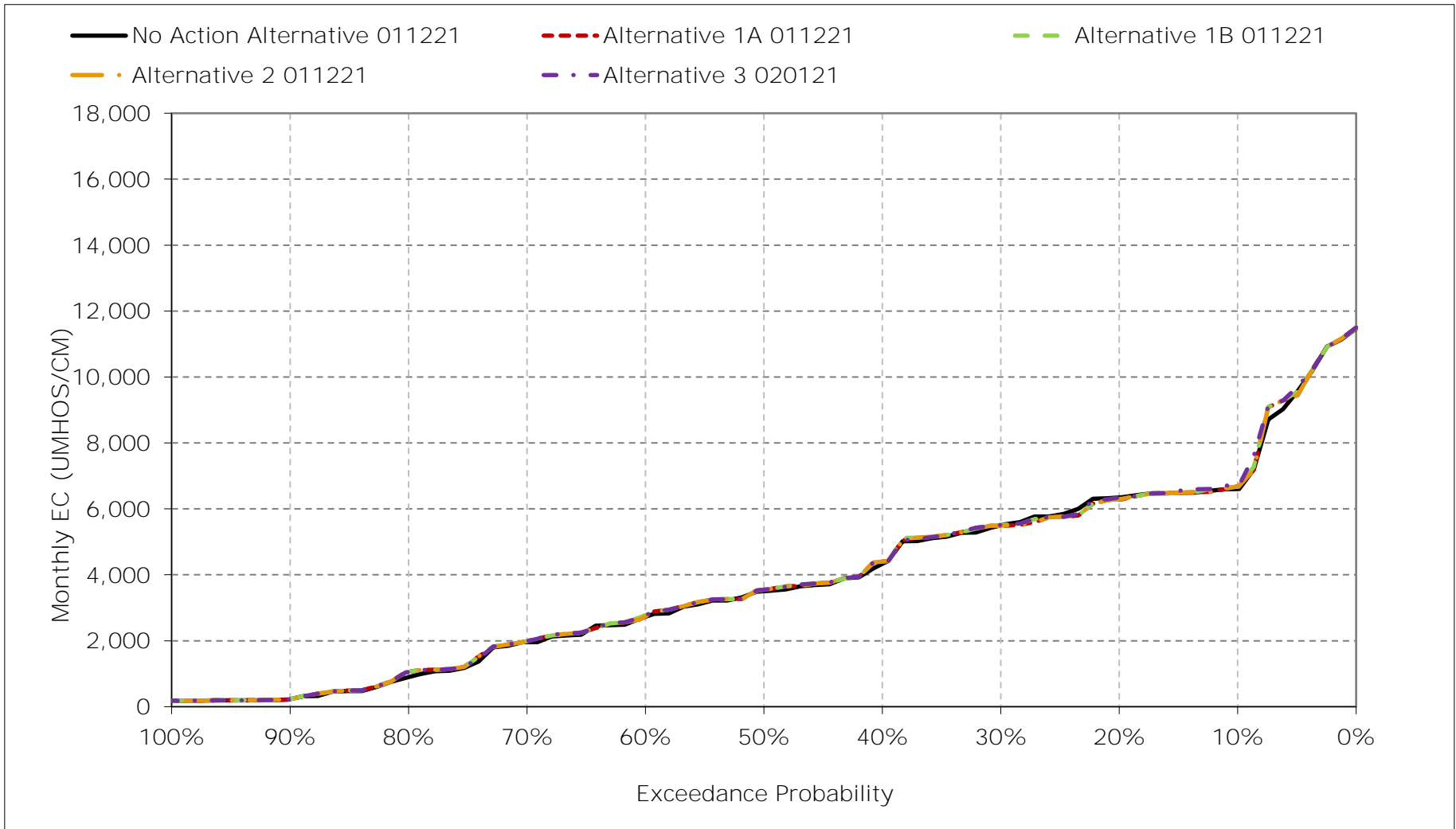
Figure 6B1-9-12. Chippis Island South Channel Salinity, June EC
