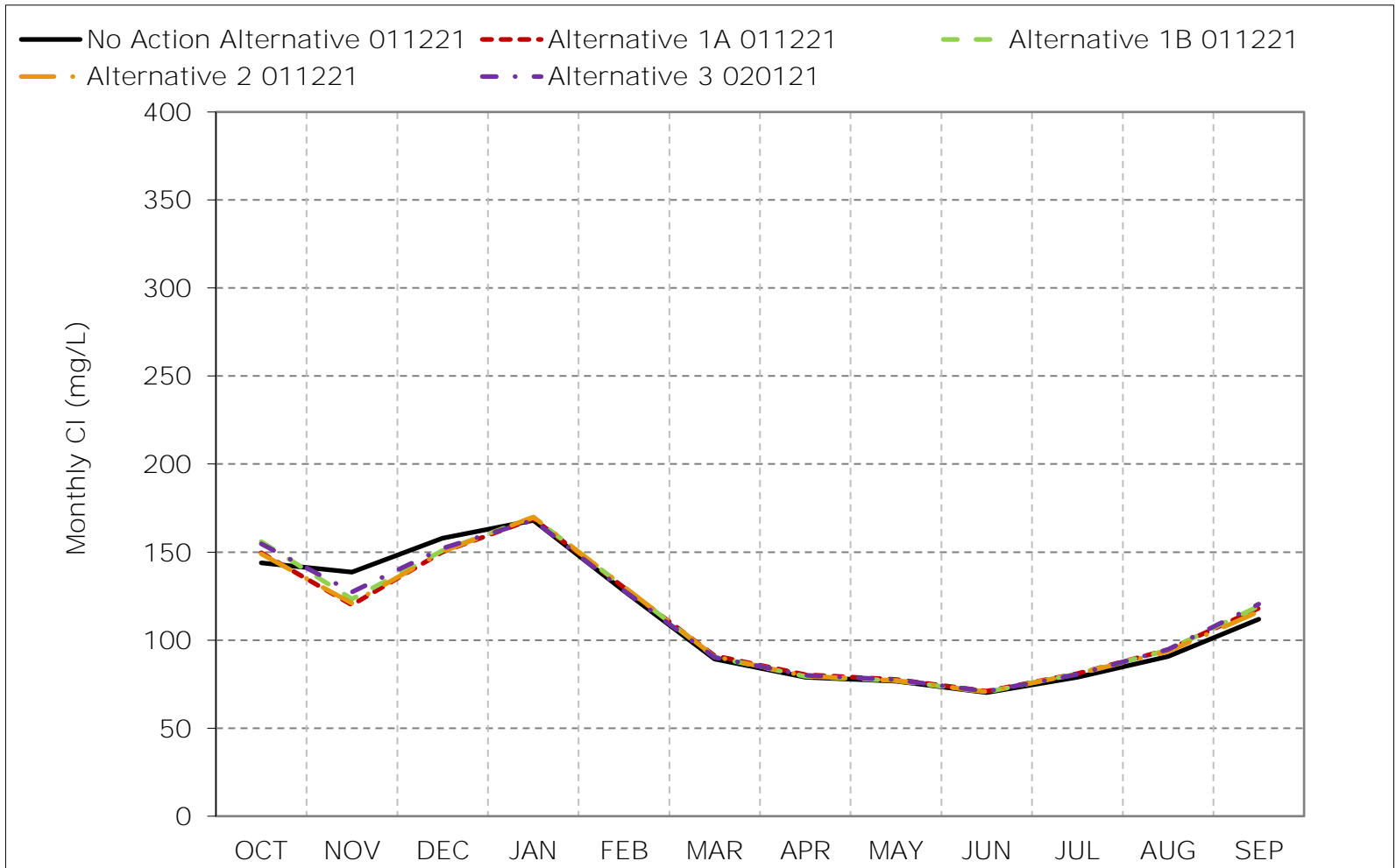
Figure 6B2-3-6. Banks Pumping Plant South Delta Exports, Critical Year Average Cl
