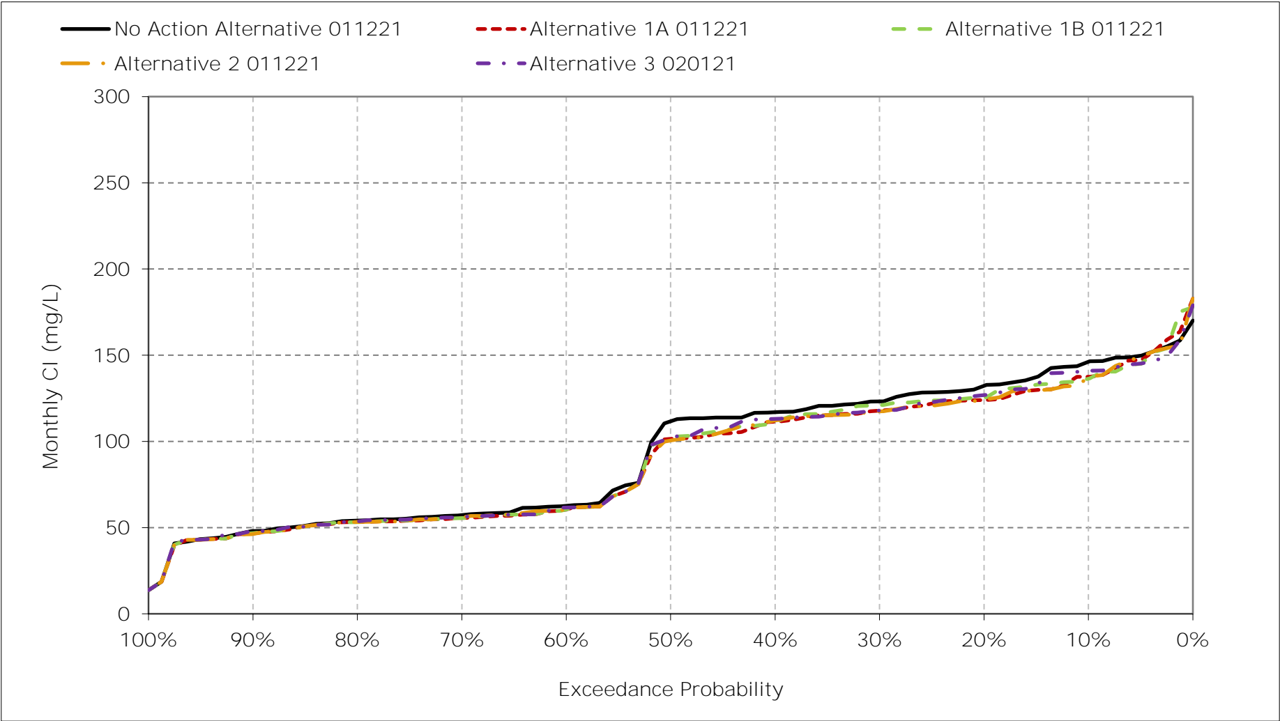
Figure 6B2-4-17. Jones Pumping Plant South Delta Exports Chloride, November CI
